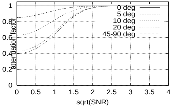
Fig. 3. A family of attenuation curves plotted versus the square root of the instantaneous SNR r . For a given SNR, attenuation increases with the angular distance between v and the orientation. Plot based on eqs. (5) and (7) for \lambda_0 = 1.5 , \alpha = 1 .
