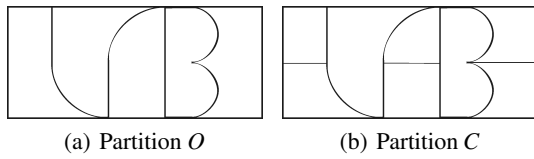
Figure 2: The right partition is a refinement of the left partition.
