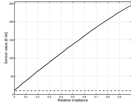
(b) Camera transfer function f of our internal gray level camera Sony XCD-SX900; solid lines denote measurements, the dotted line is a line fit, and the dashed line marks the black level.
