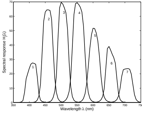
(a) Joint spectral characteristics H_i(\lambda) of optical bandpass filters \tau_i(\lambda) and sensor R(\lambda) .
